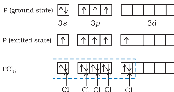
sp 3 d hybrid orbitals filled by electron pairs donated by five Cl atoms.
